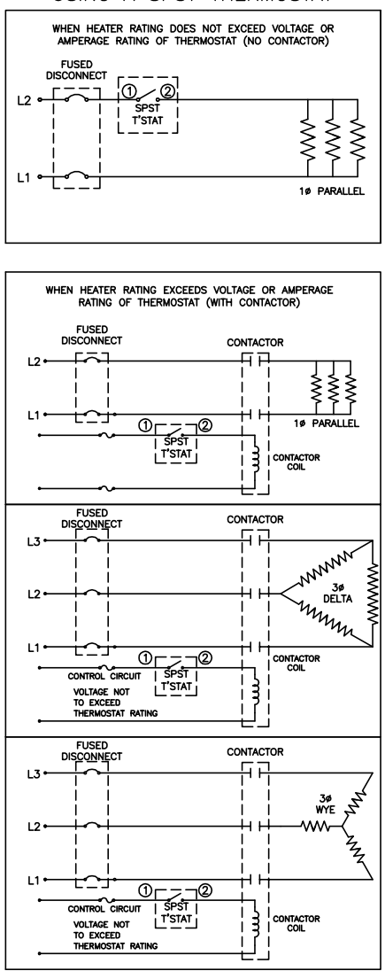
TYPICAL WIRING WITH 3 ELEMENTS USING A SPST THERMOSTAT
