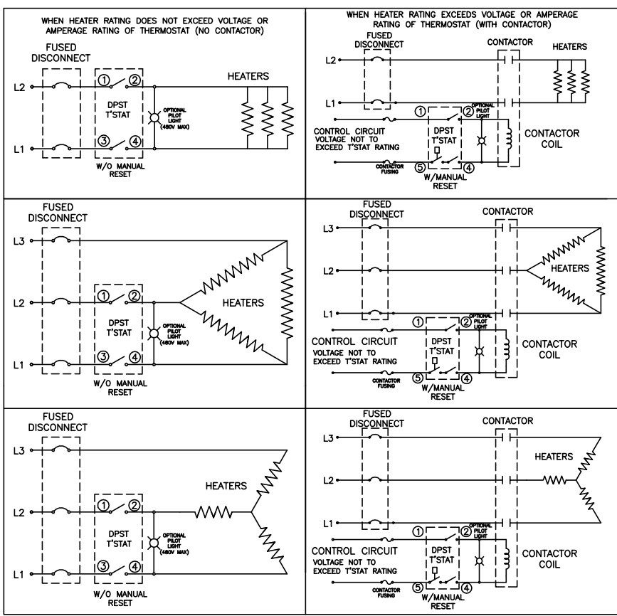
TYPICAL WIRING WITH 3 ELEMENTS USING A DOUBLE POLE THERMOSTAT
